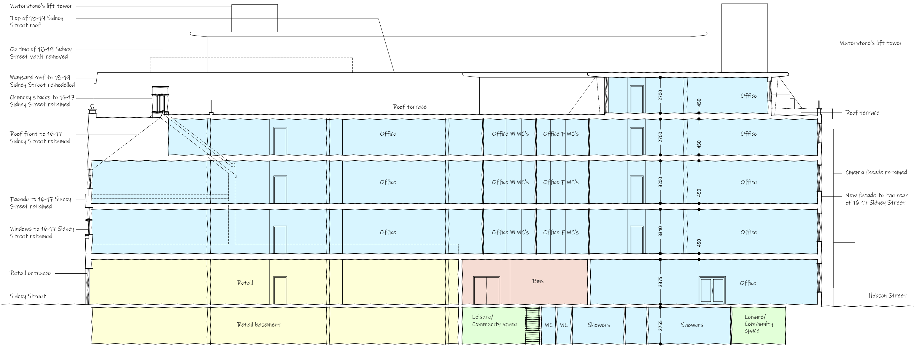
LONG SECTION "BB" THROUGH 16 - 17 SIDNEY STREET
