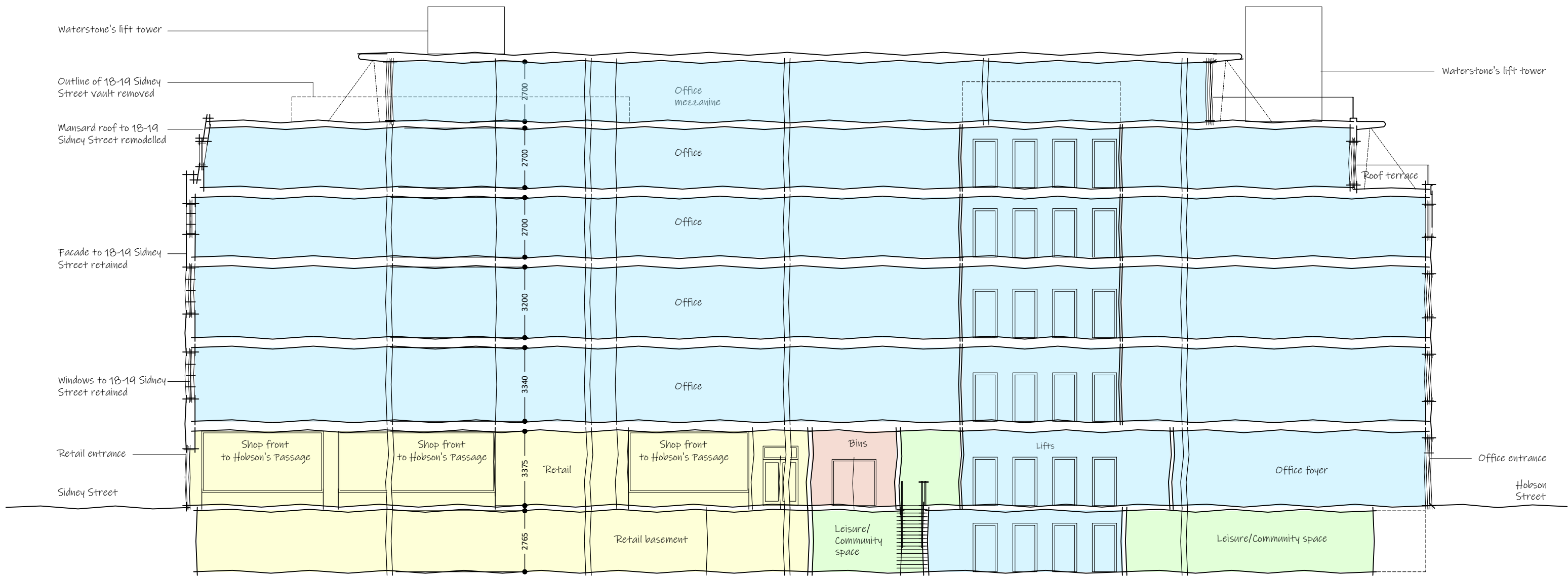
LONG SECTION "BB" THROUGH 18 - 19 SIDNEY STREET
