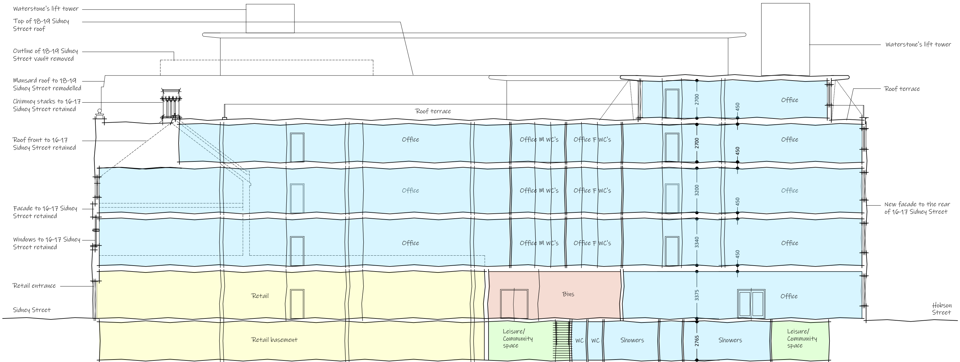
LONG SECTION "AA" THROUGH 16 - 17 SIDNEY STREET
